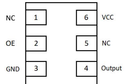
Pin Assignments
