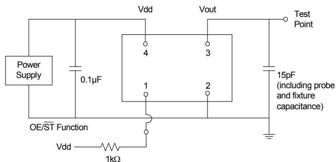
Figure 1. Test Circuit
