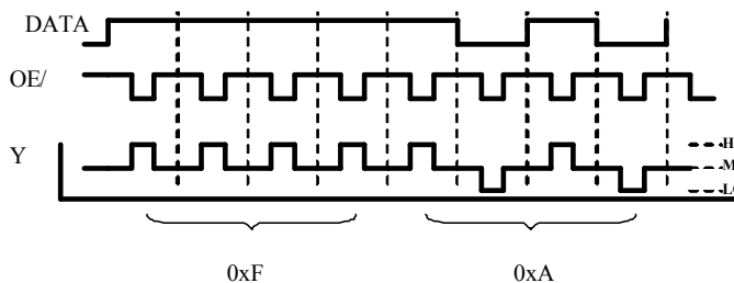
Figure 8. Signal Polarity
