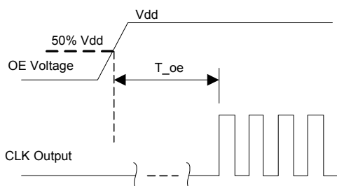
T_oe: Time to re-enable the clock output
