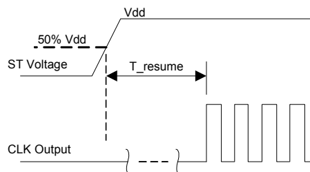
T_resume: Time to resume from ST
