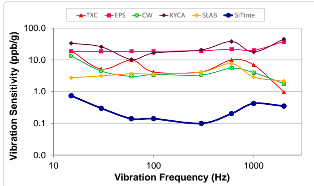
Figure 5. Vibration Robustness [5]
