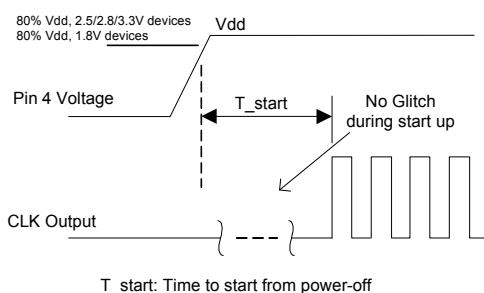
T_start: Time to start from power-off
